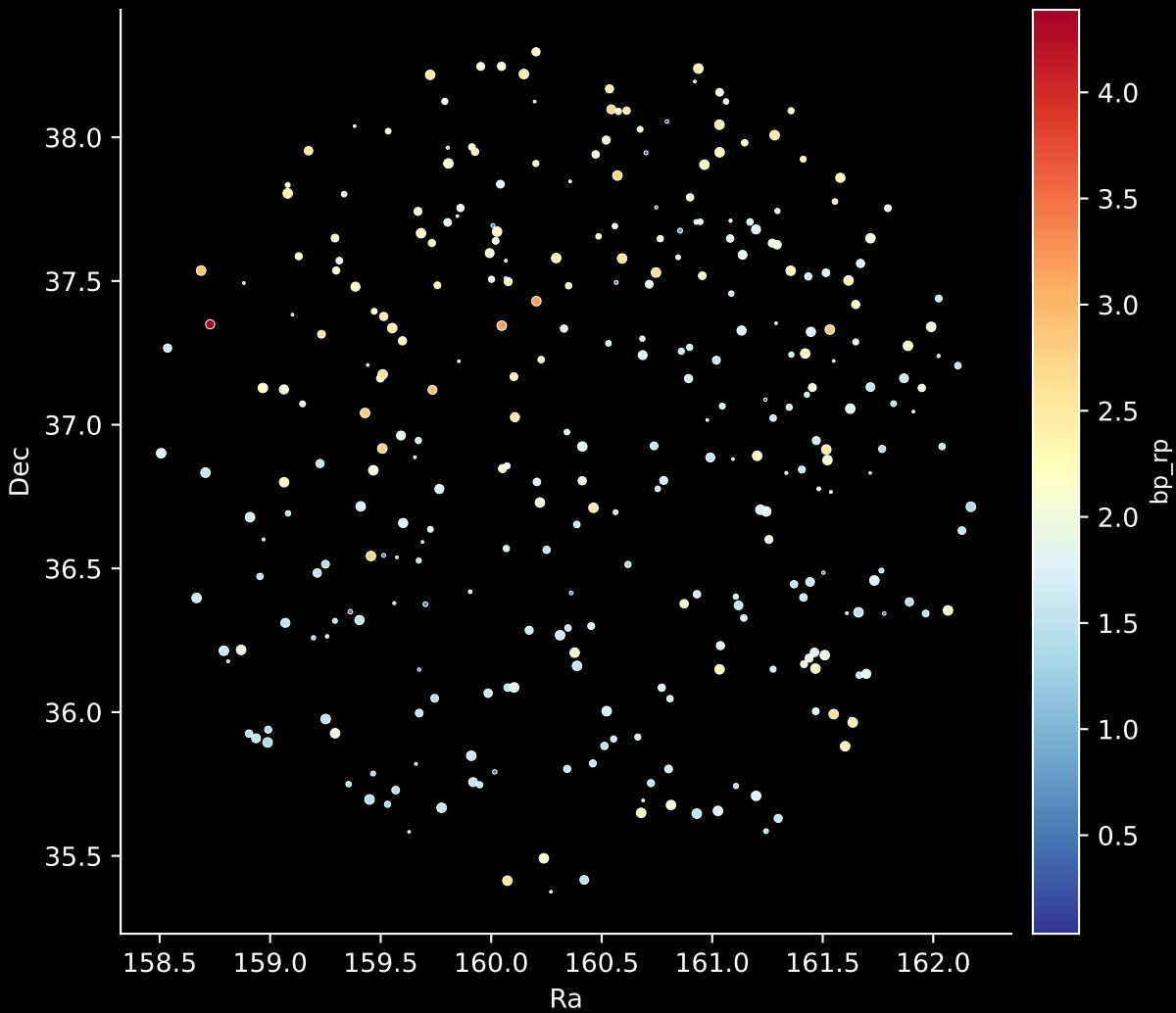
APOGEE DR17 Field: [160-12] Stars: 311
