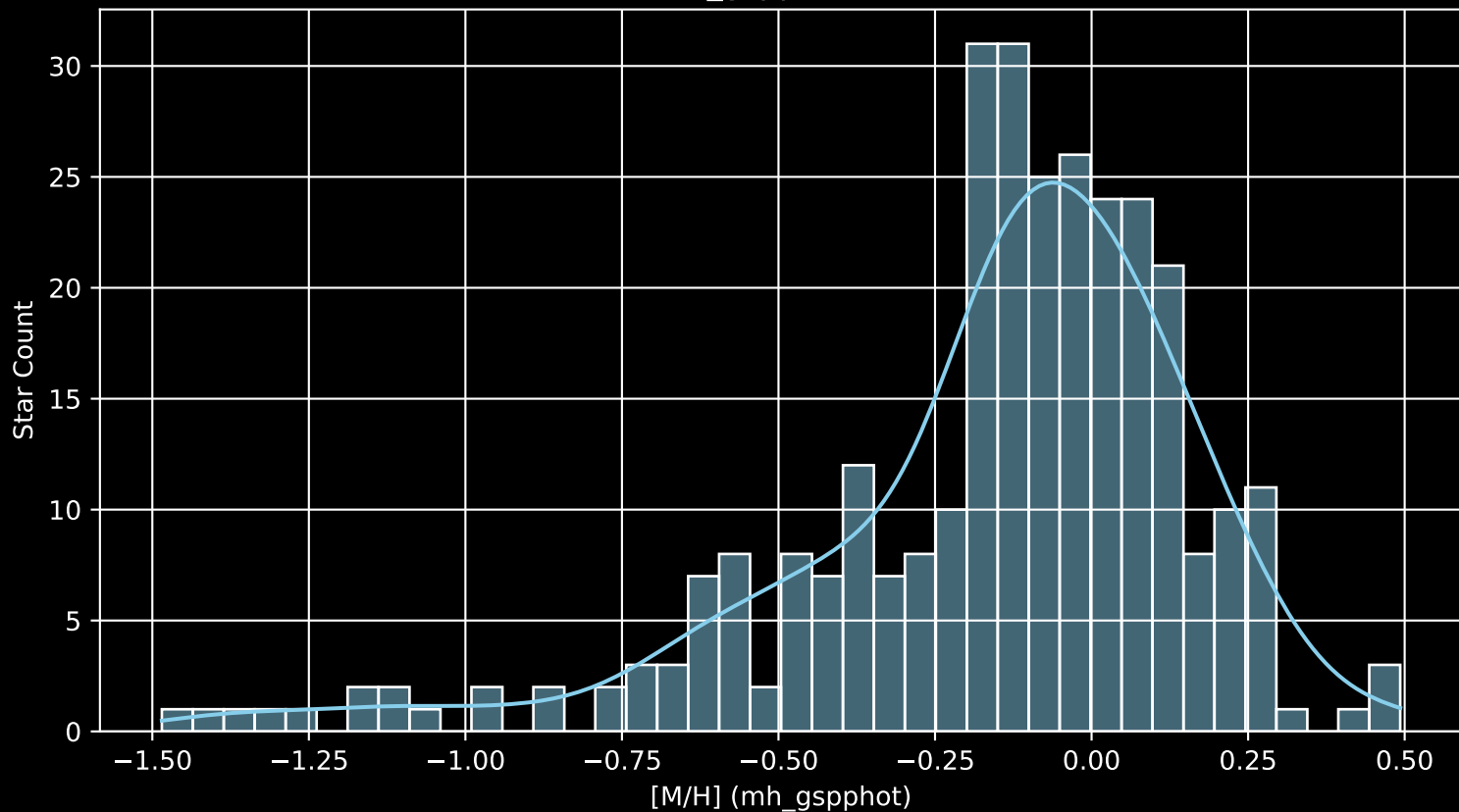
APOGEE DR17 Field: [160-12 [M/H] (mh_gspphot) (n= 307)
