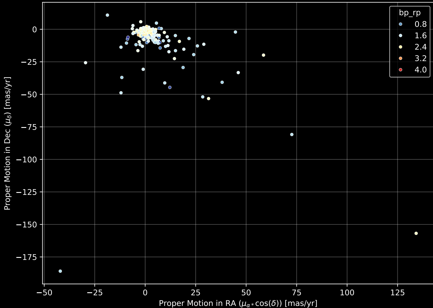
APOGEE DR17 Field: [160-12] Proper Motion Diagram (n= 311)
