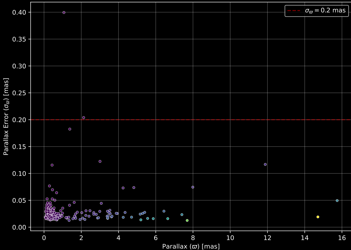
APOGEE DR17 Field: [160-12] Parallax Quality (n= 311)
