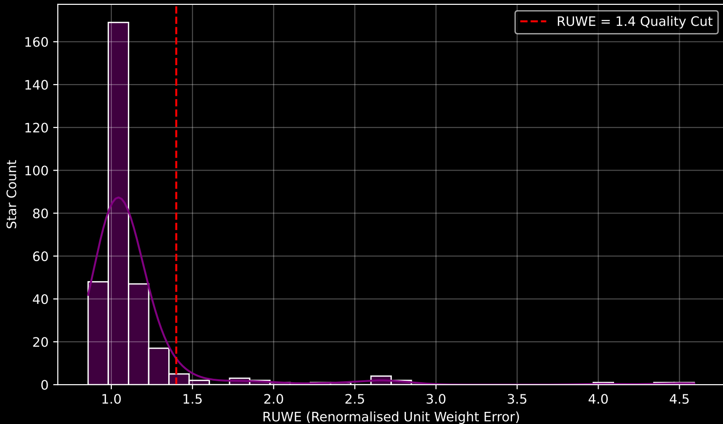
GAPOGEE DR17 Field [160-12] RUWE Distribution (n= 305)
