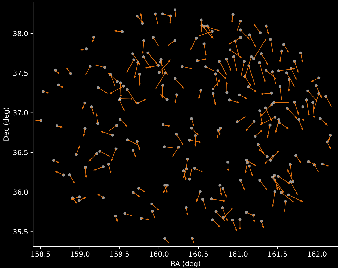
APOGEE DR17 Cluster 2 Proper Motion Vectors (n=210)
